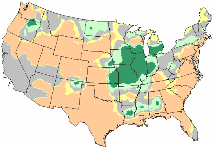
Weekly Rainfall vs Normal (20 JUN 2010 - 26 JUN 2010)
