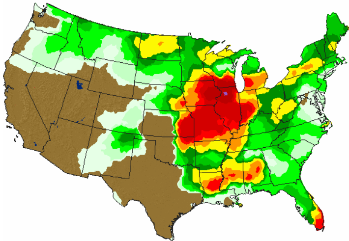
Weekly Rainfall (20 JUN 2010 - 26 JUN 2010)
