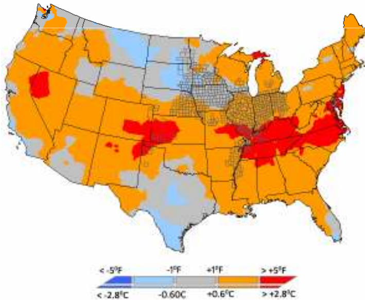
Weekly Max Temperature vs Normal (19 JUL 2010 - 25 JUL 2010)
