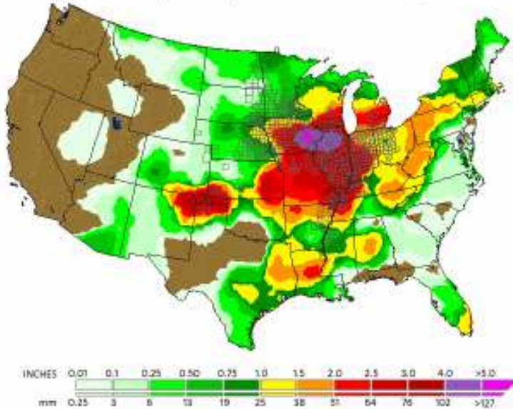
Weekly Rainfall (19 JUL 2010 - 25 JUL 2010)
